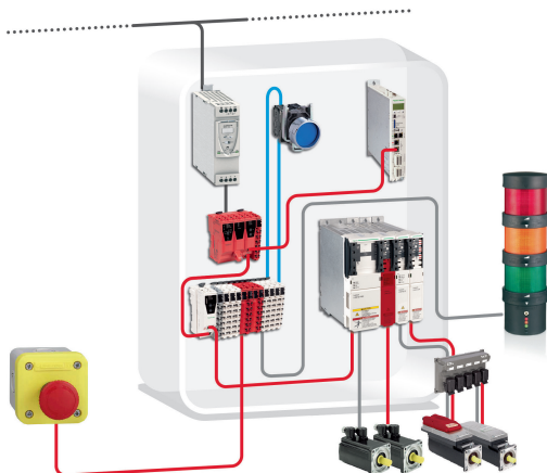
Example of Safety architecture with Modicon TM5CSLC Safety logic controller, Modicon TM5 safety & non-safety expansion modules, integrated drives and safety module for a safe communication over Sercos automation bus.
